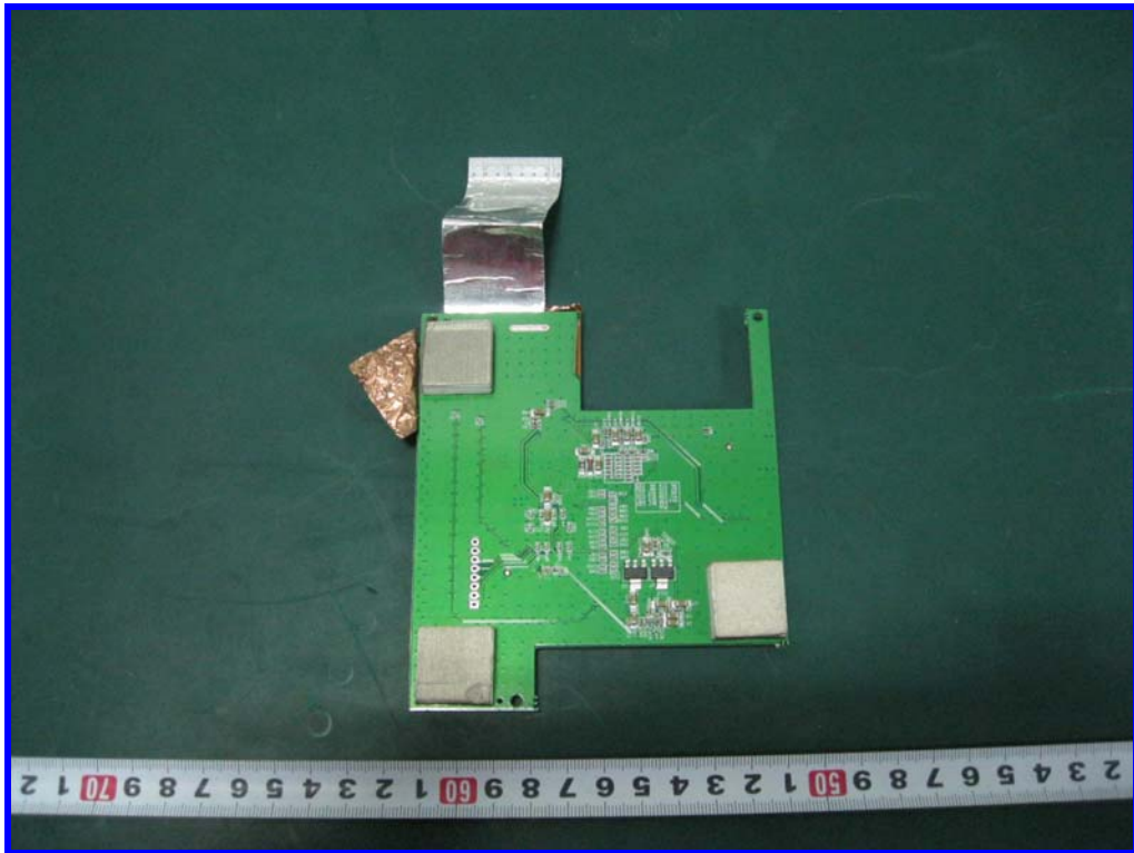
Photo #11 EUT-Front View of PCB
