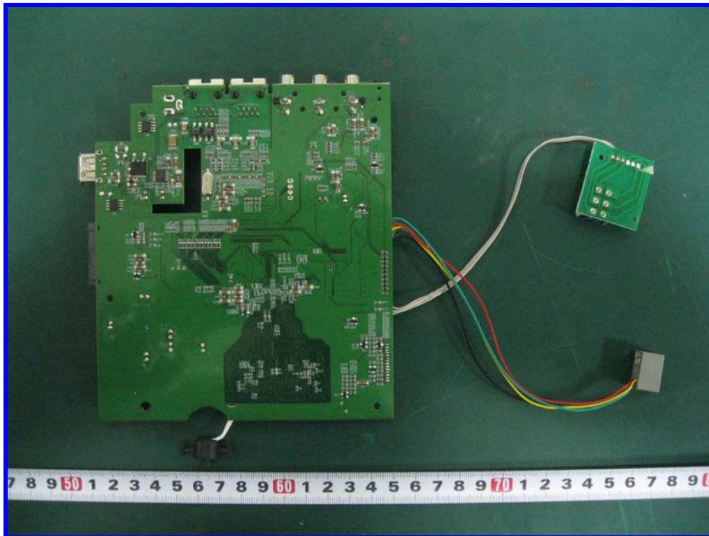
Photo #3 EUT-Rear View of Main PCB
