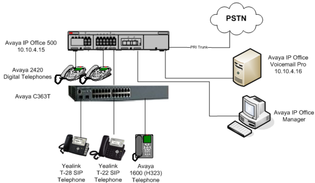
Figure 2 – Test Configuration
