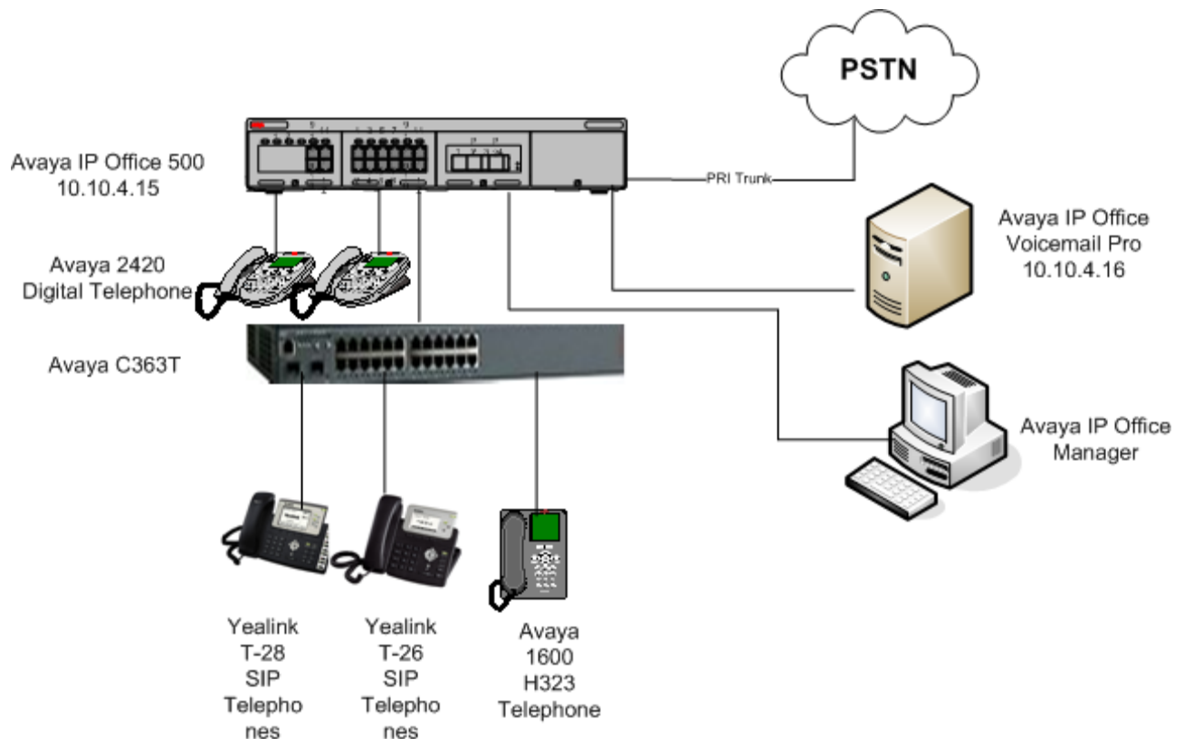
Figure 2 – Test Configuration
