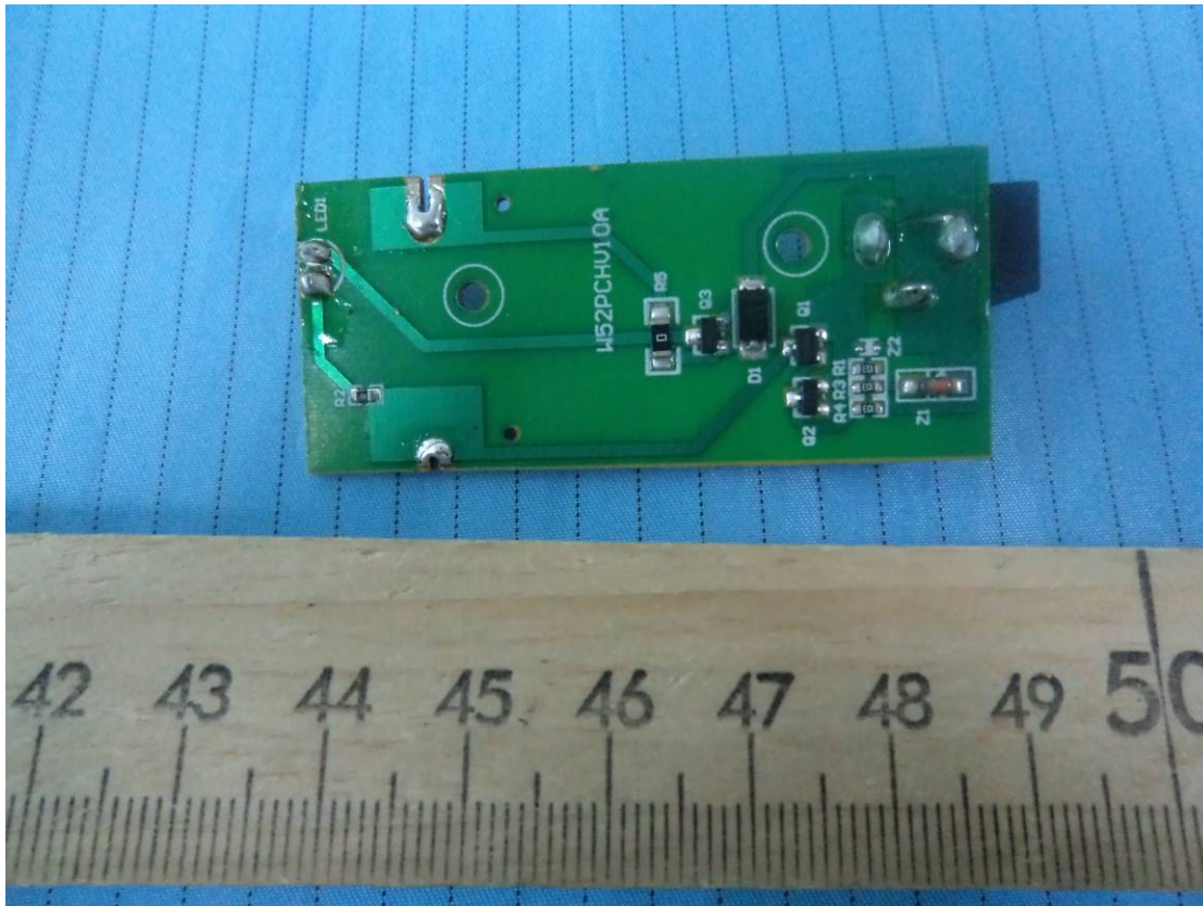
A.17 EUT- Top view of PCB of charger
