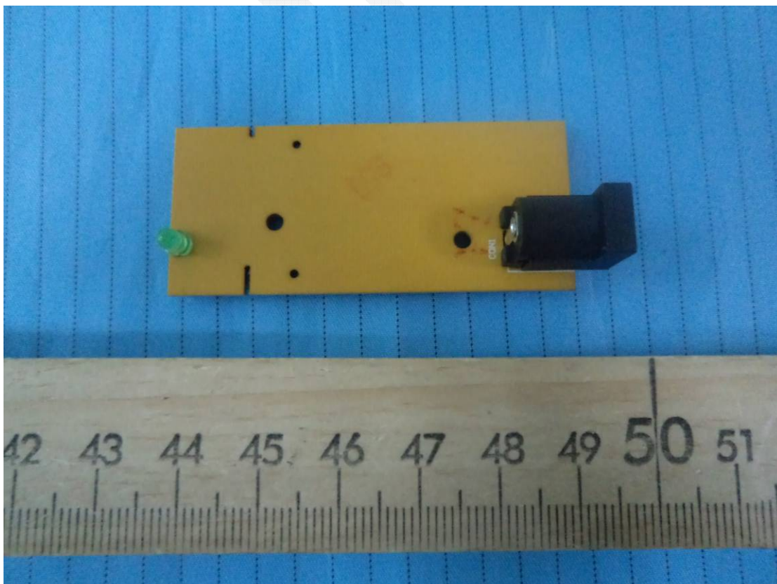
A.18 EUT- Bottom view of PCB of charger
